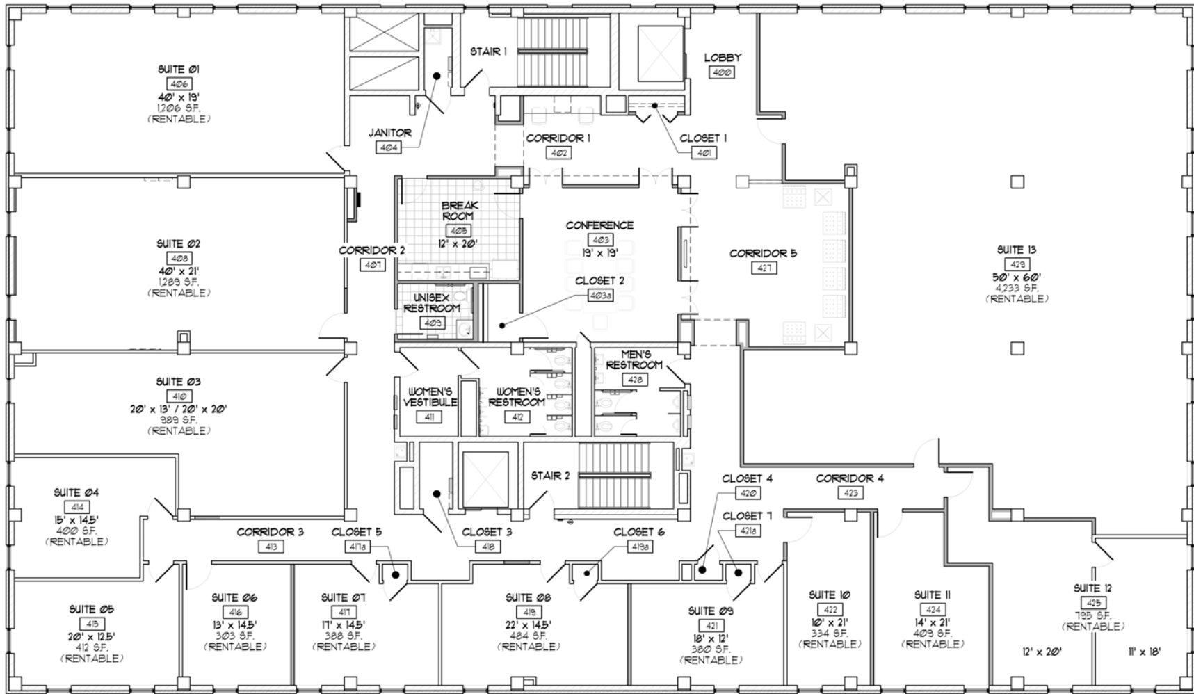
A BUILDING 'C' - FOURTH FLOOR PLAN SCALE: 3/32" = 1'-0"
